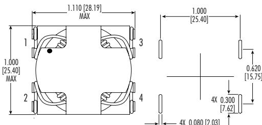
SUGGESTED PAD LAYOUT
