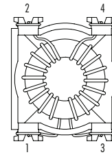
BOTTOM VIEW
